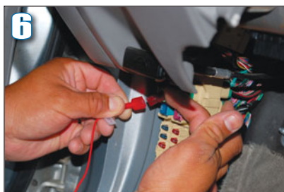
6 Make power, ground and accessory connections. Solder or use T-taps on pre-tested and verified wires. Note: no reverse input required; the screen switches to rear-camera view when it sends a video signal at the input.
